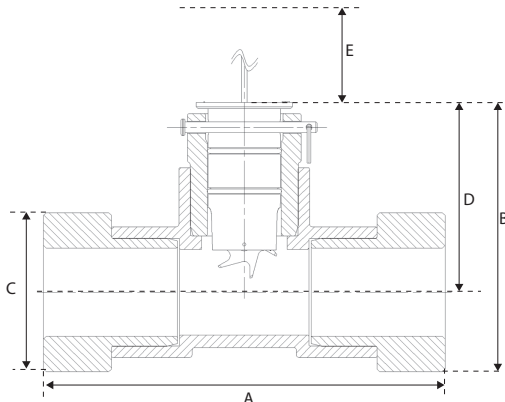
BSP Fittings
