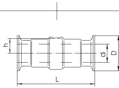
Neumo BioConnect clamp connection
