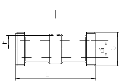
Neumo BioConnect connection thread
